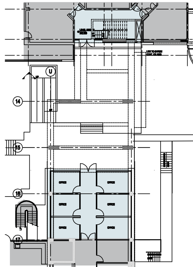
8000 LEVEL PLAN
