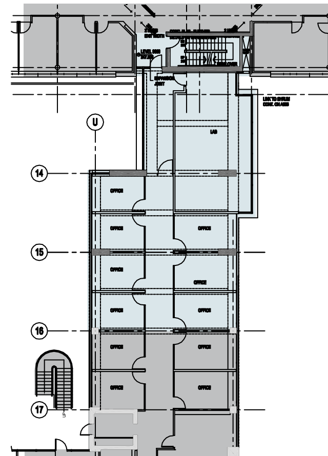
9000 LEVEL PLAN
