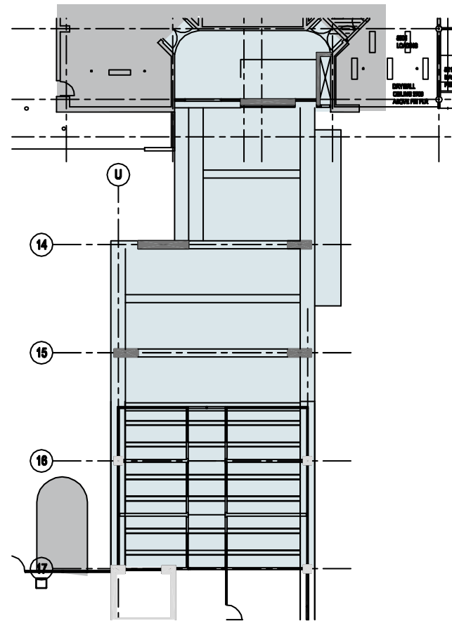
8000 LEVEL RCP
