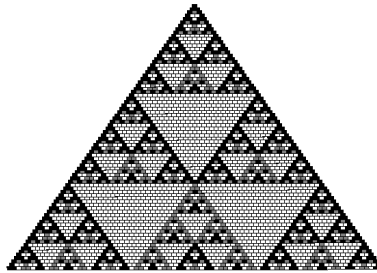
Figure 6: Eighty rows of Pascal's Triangle mod 3
