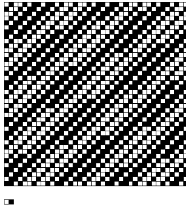
Figure 10: Integer part of \{ie\}_{i=1}^{1600} \bmod 2 ; note the slight irregularities in the pseudo-periodic pattern.
