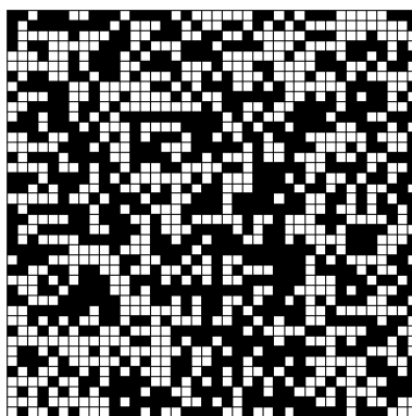
Figure 2: The first 1600 decimal digits of \pi \bmod 2 .
