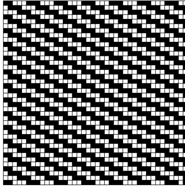
Figure 3: The first 1600 decimal digits of 22/7 \bmod 2 .
