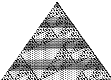
Figure 7: Eighty Chebyshev Polynomials mod 3
