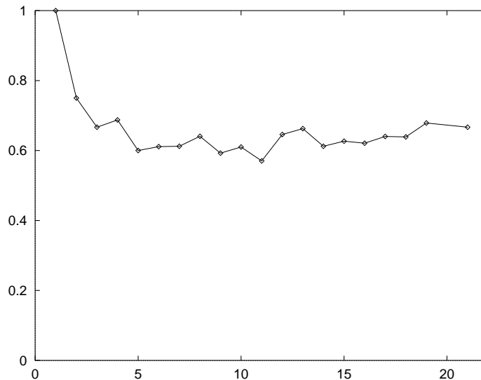
FIGURE 1. d/m^2 versus m for height 1 multiples of (x - 1)^m of smallest known degree.
