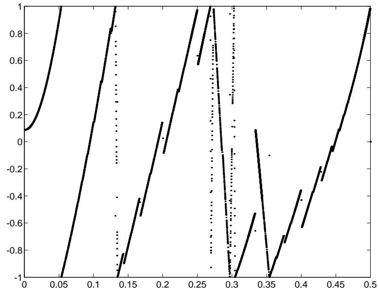
Figure 6: A_{J(\phi)} against \phi/\pi for g = 1 .
