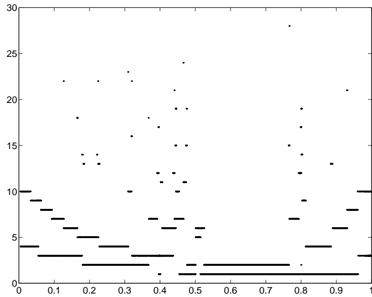
Figure 10: I, J against \phi/\pi for g = 1 .
